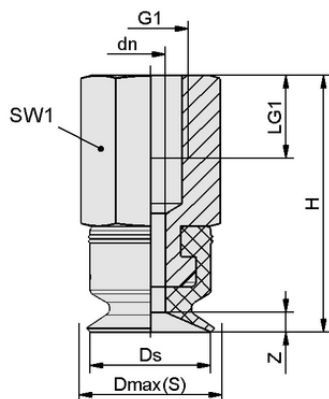
Design data PFYN 5 SI-CO-55 M5-IG
