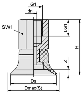
Design data PFYN 50 NBR-CO-55 G1/8-IG
