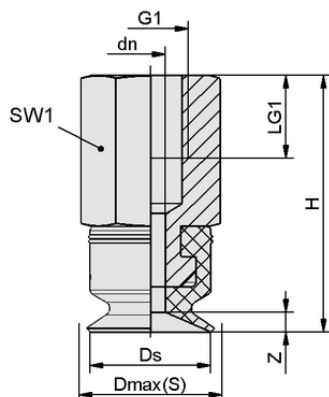
Design data PFYN 10 NBR-CO-55 M5-IG
