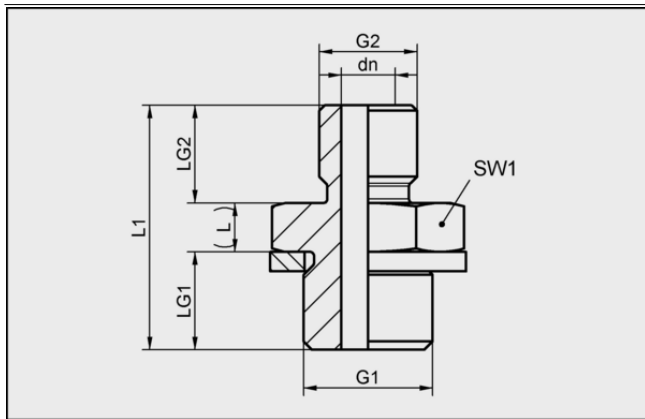
Design data SA-NIP N009 G1/4-AG
