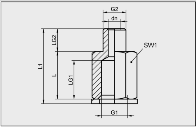
Design data SA-NIP N009 G1/4-IG
