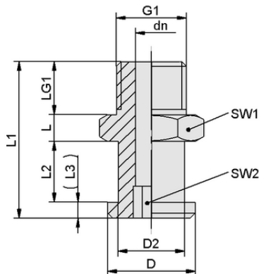
Design data SA-NIP N006 G1/8-AG DN200
