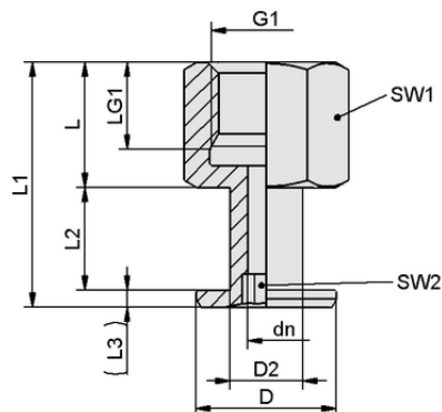
Design data SA-NIP N008 G1/8-IG DN350
