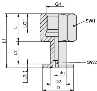
Design data SA-NIP N006 G1/8-IG DN200
