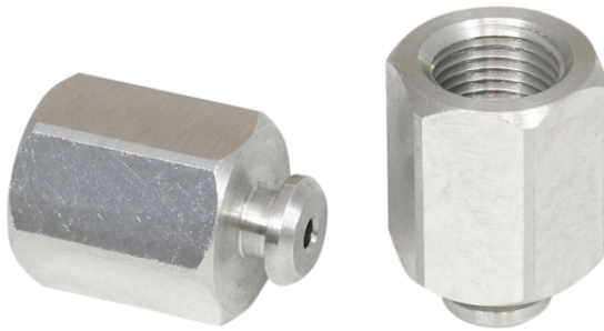
SA-NIP N005 G1/8-IG DN200
