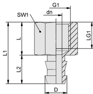
Design data SA-NIP N033 G1/4-IG DN550
