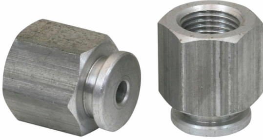
SA-NIP N029 G1/8-IG DN350
