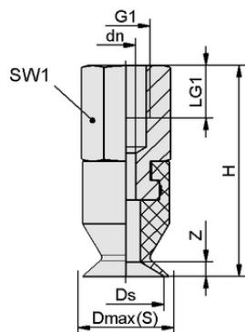
Design data SGAN 16 SI-55 G1/8-IG
