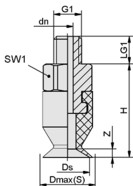
Design data SGAN 13 PU-60 G1/8-AG
