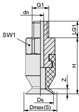
Design data SGAN 13 SI-55 G1/8-AG
