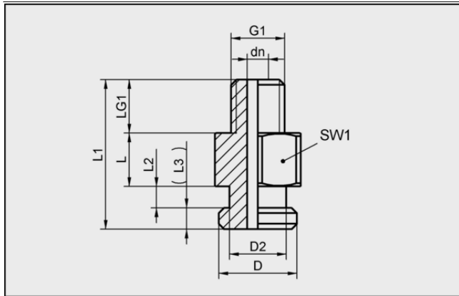
Design data SA-NIP N028 M5-AG DN200
