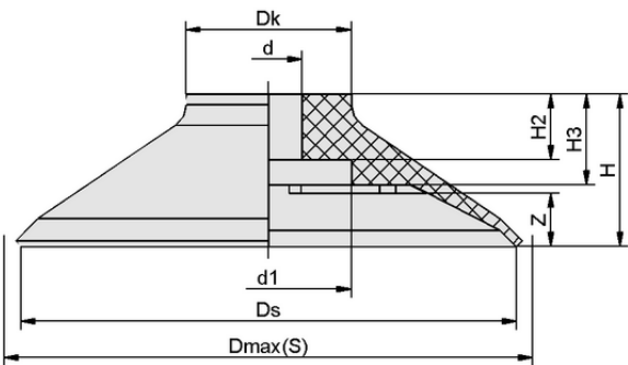
Design data PFG 50 VU1-72 N011
