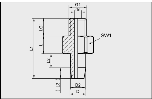
Design data SA-NIP N055 M3-AG DN100
