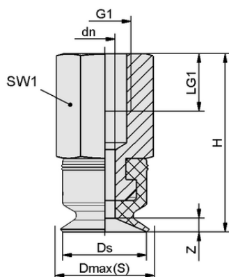
Design data PFYN 10 NBR-55 G1/8-IG
