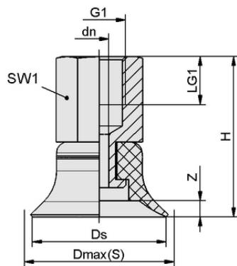
Design data PFYN 25 FPM-65 G1/8-IG
