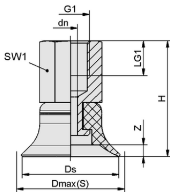
Design data PFYN 20 NBR-55 G1/8-IG
